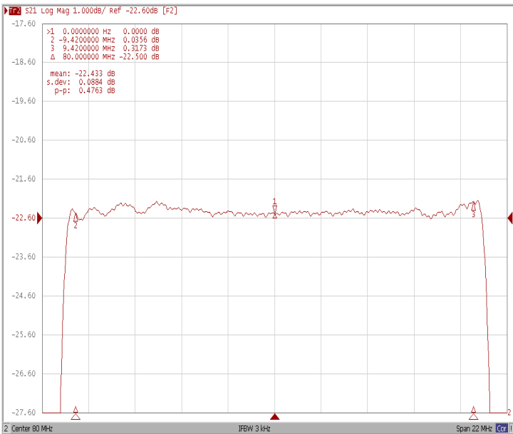
Ripple Variation Fo±9.42Hz
